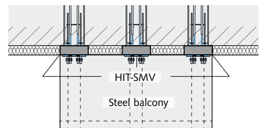
Application: Cantilever balcony
